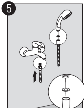
请注意密封垫圈的使用 Check that both ends of hose include rubber washers
